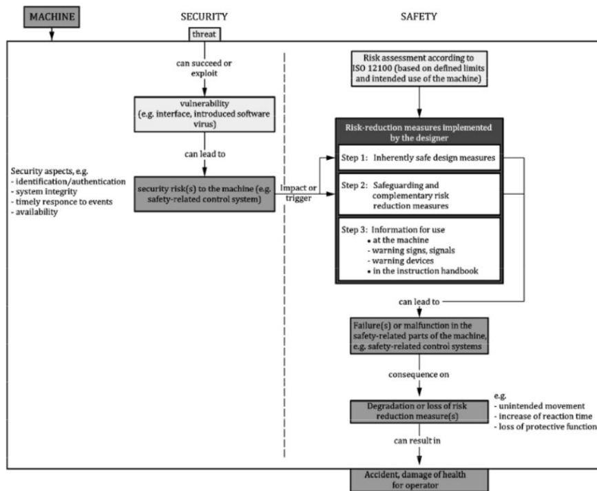
Relationship between safety of machinery and cybersecurity
